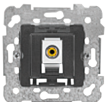
RCA video socket outlet 18577 Rear screw-less terminal Cable: maximum 3 pairs of 0.3 mm 2
