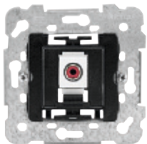
Mono RCA socket outlet 18575 Rear screw-less terminal Cable: maximum 3 pairs of 0.3 mm 2
